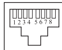
Modular 8-pin
